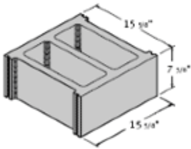
16 x 8 x 16 Hollow Stretcher
