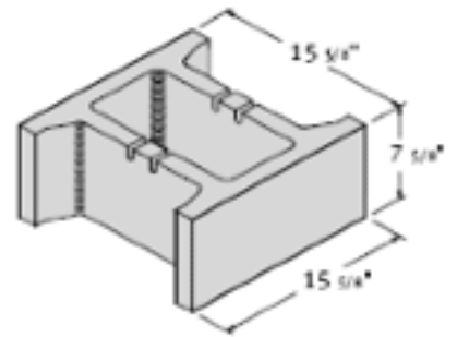
16 x 8 x 16 Ivory (Rebar) Block
