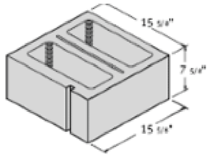
16 x 8 x 16 Hollow Corner Sash
