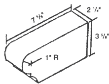
Step Tread SS-OGH
